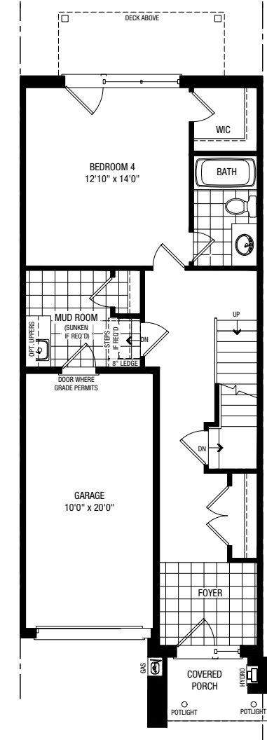
OPT. GROUND A 4 BEDROOM PLAN
